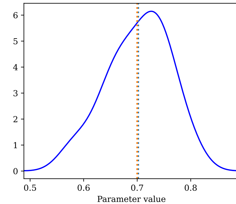
G shock AR(1)
