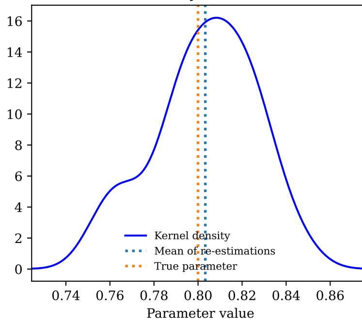
Productivity shock AR(1)
